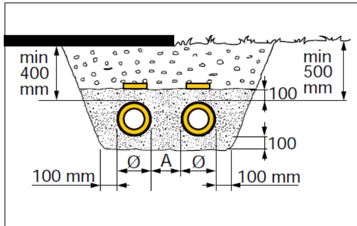
Figure 32: Indicative Trench Dimensions (source: Logstor Design Manual)
