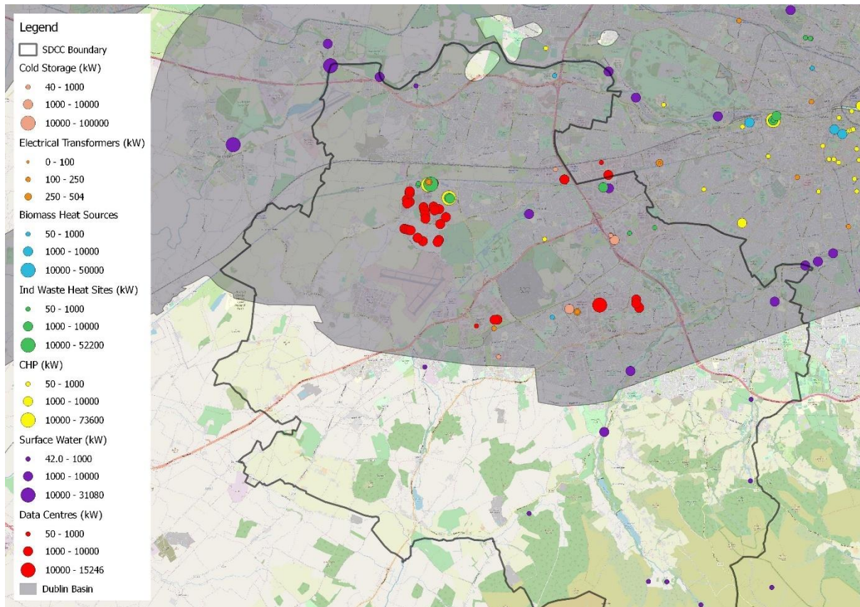
Figure 19: South Dublin Heat Source Map
