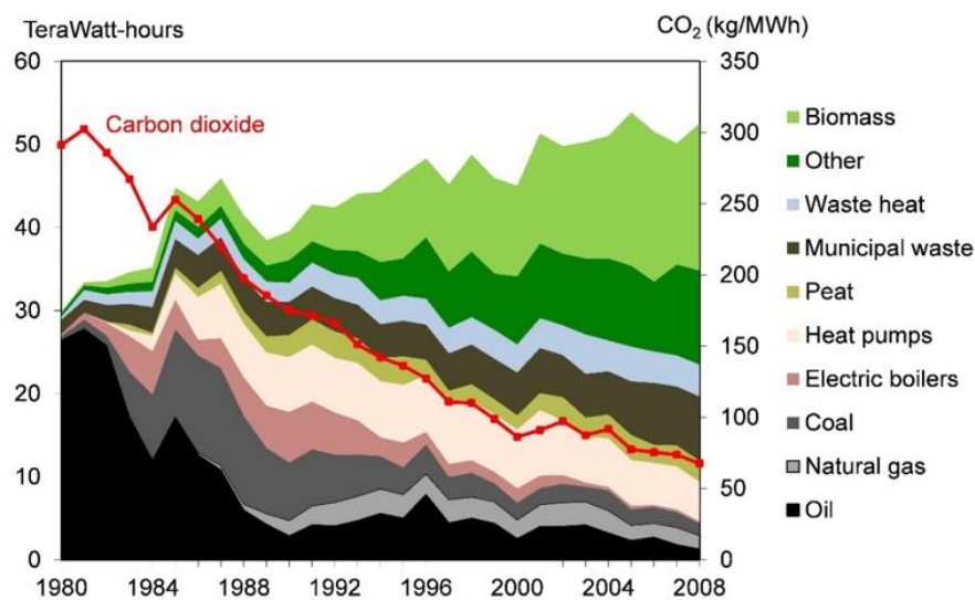
Figure 11: Fuel Sources and Emissions in Swedish District Heating Systems (Source: Nordic Heating & Cooling 2017)
