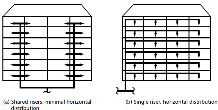
Figure 33: Shared Riser Diagram (Source: CIBSE Heat Networks Code of Practice)
