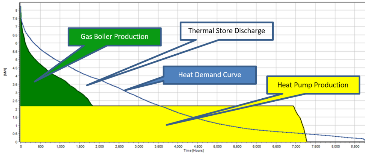
Figure 26: Example of Plant Size Modelling – Heat Production & Duration Curve
