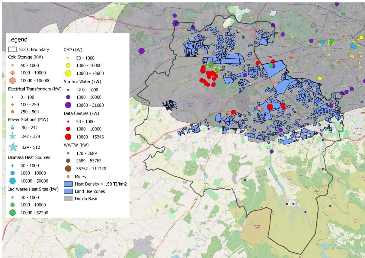
Figure 18: Combined Heat Source, Heat Demand and Relevant Development Zone (RES-N, REGEN & SDZ) Map
